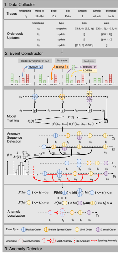
Figure 1: TFOW consists of three modules: (i) data collector; (ii) Event constructor; and (iii) anomaly detector. Note, (a, b) here is not an event but the actual price and depth.
